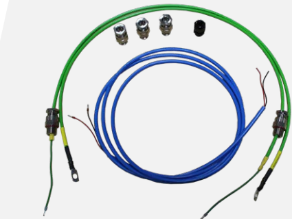
Kit B - with Ex d glands, for use with non-armoured cable
