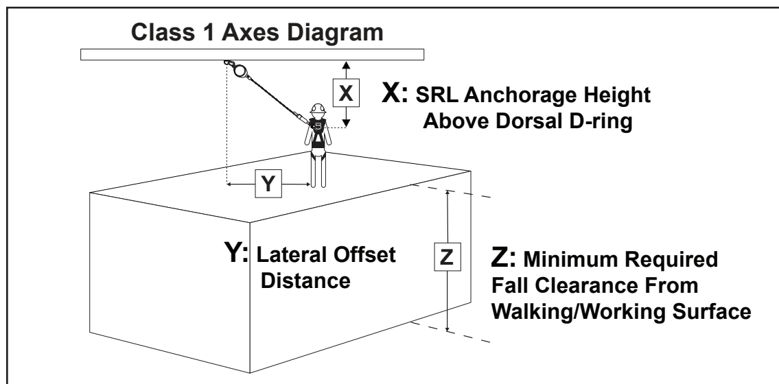
FIGURE 1 - CLASS 1 SRL AXES DIAGRAM
