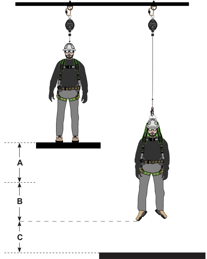
FIGURE 2 - EXAMPLE MINIMUM REQUIRED FALL CLEARANCE CALCULATION (CLASS 1 SRL)
