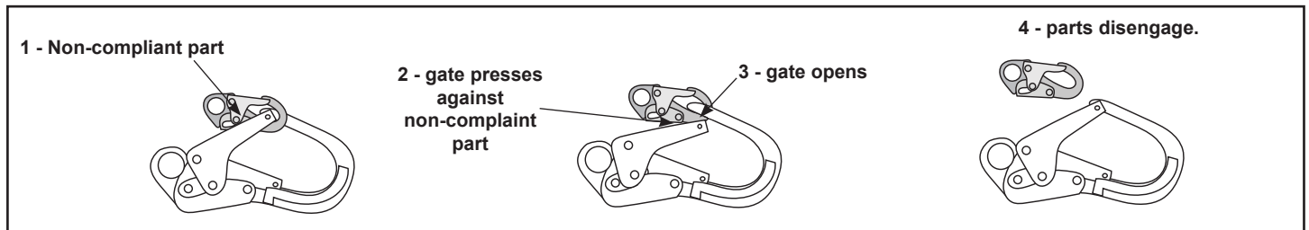
FIGURE 5 - UNINTENTIONAL DISENGAGEMENT
