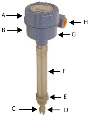
Figure 1. Rosemount 2130 Features
