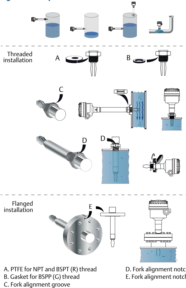
Figure 5. Example Installations
