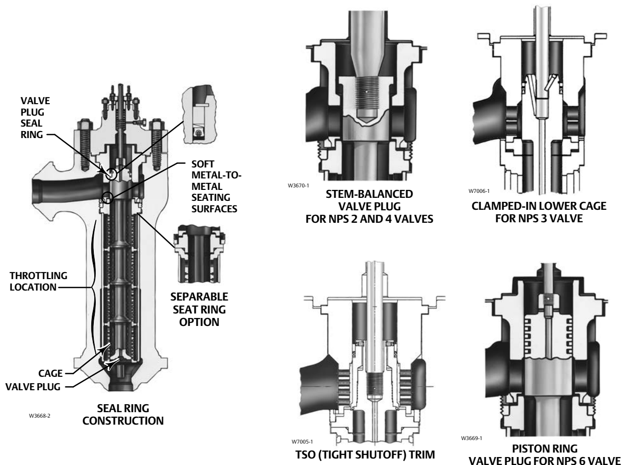
Figure 1. Sectional View of Fisher CAV4 Valve Body with Cavtrol IV Trim
