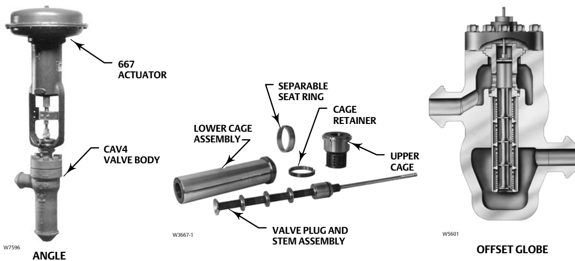
Fisher 657-CAV4 Control Valve Assembly with Cavitol IV Trim
