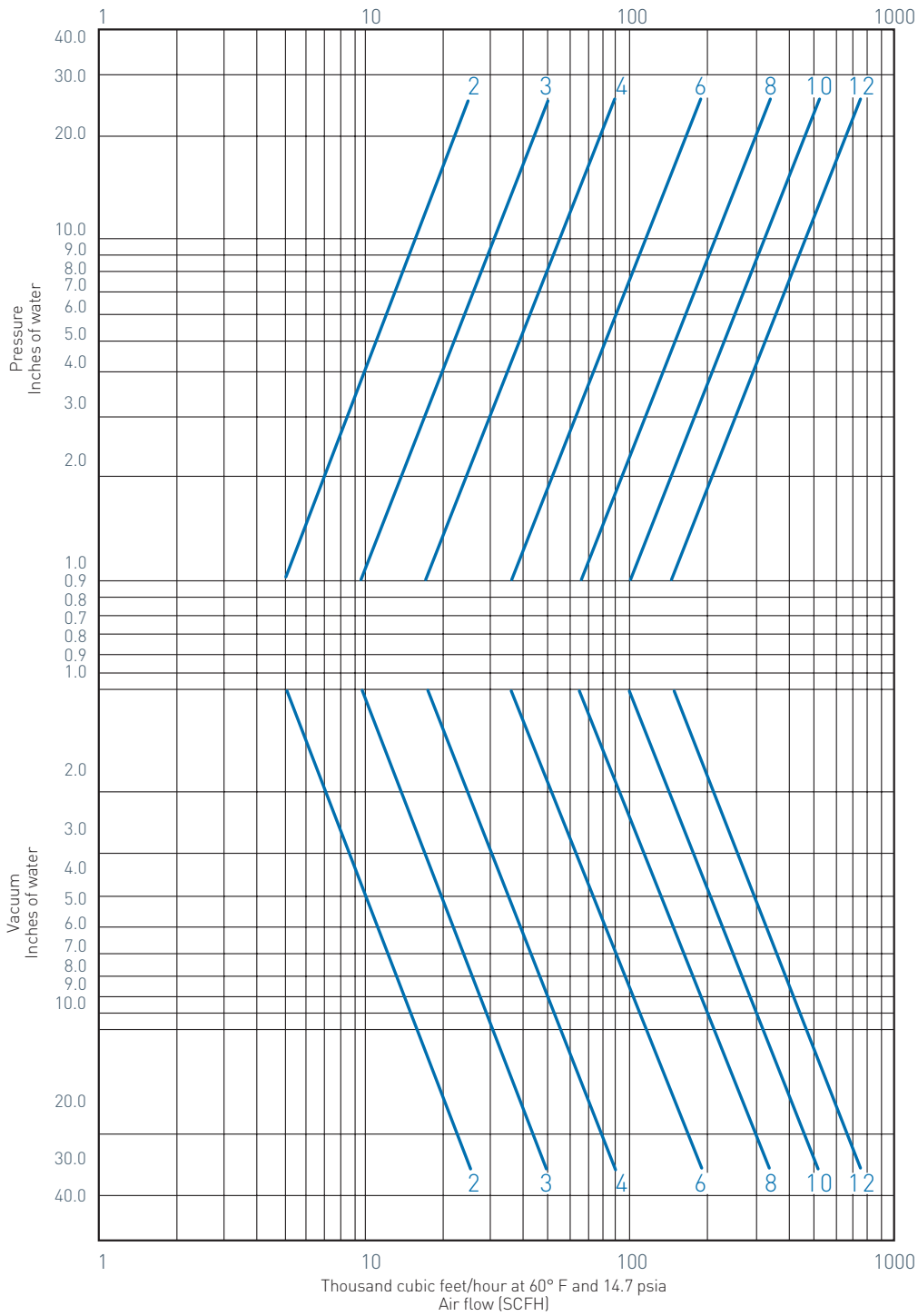
FIGURE 7000 FREE VENTS
