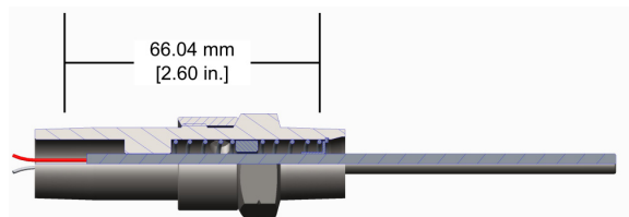
Figure 13. Dimensions
