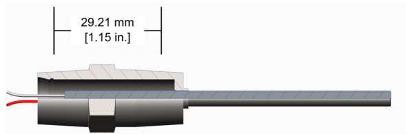
Figure 15. Dimensions
