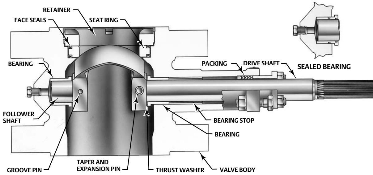
Figure 2. Sectionals of Fisher CV500 Rotary Control Valves
