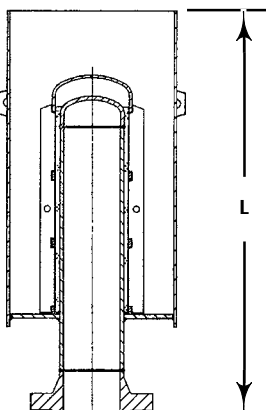
Figure 6. Fisher 6013 Vent Diffuser Dimensions
