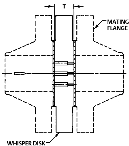
Figure 4. Thickness Dimension T for Whisper Disk Diffusers
