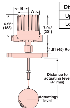
Model T20 with flange
