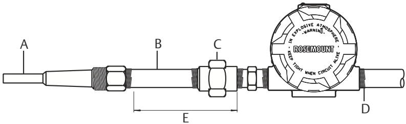
Figure 2-1: Typical Direct-Mounted Configuration
