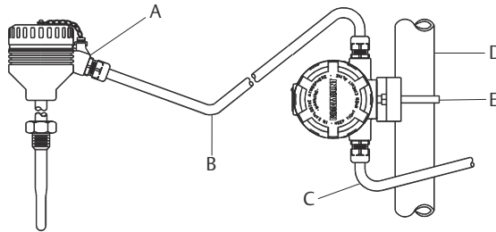
Figure 2-2: Typical Remote-Mounted Configuration with Cable Glands
