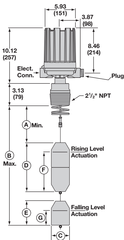
Model A10 with Threaded Mounting
