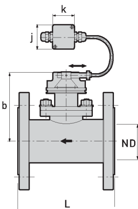
DW 183 HT side view
